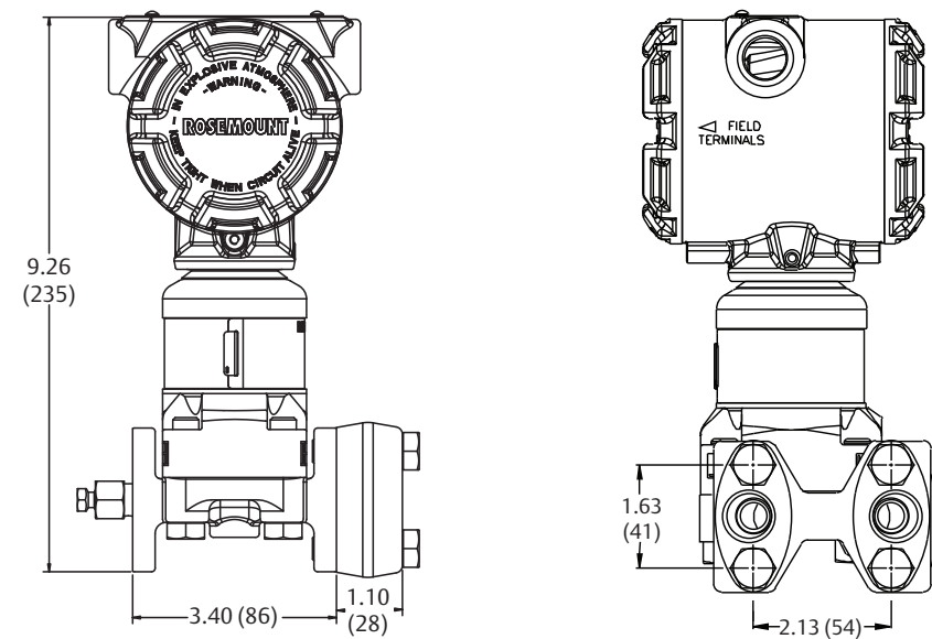
Figure 2. Transmitter with Coplanar Sensor Module and Traditional Flange
