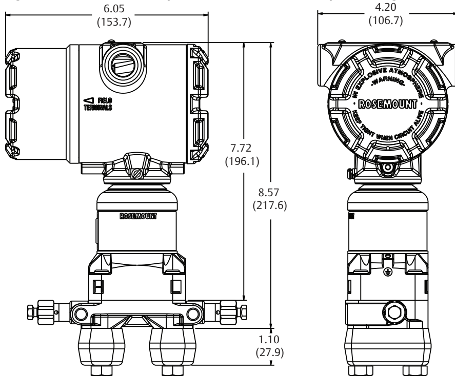
Figure 1. Transmitter with Coplanar Sensor Module and Coplanar Flange
