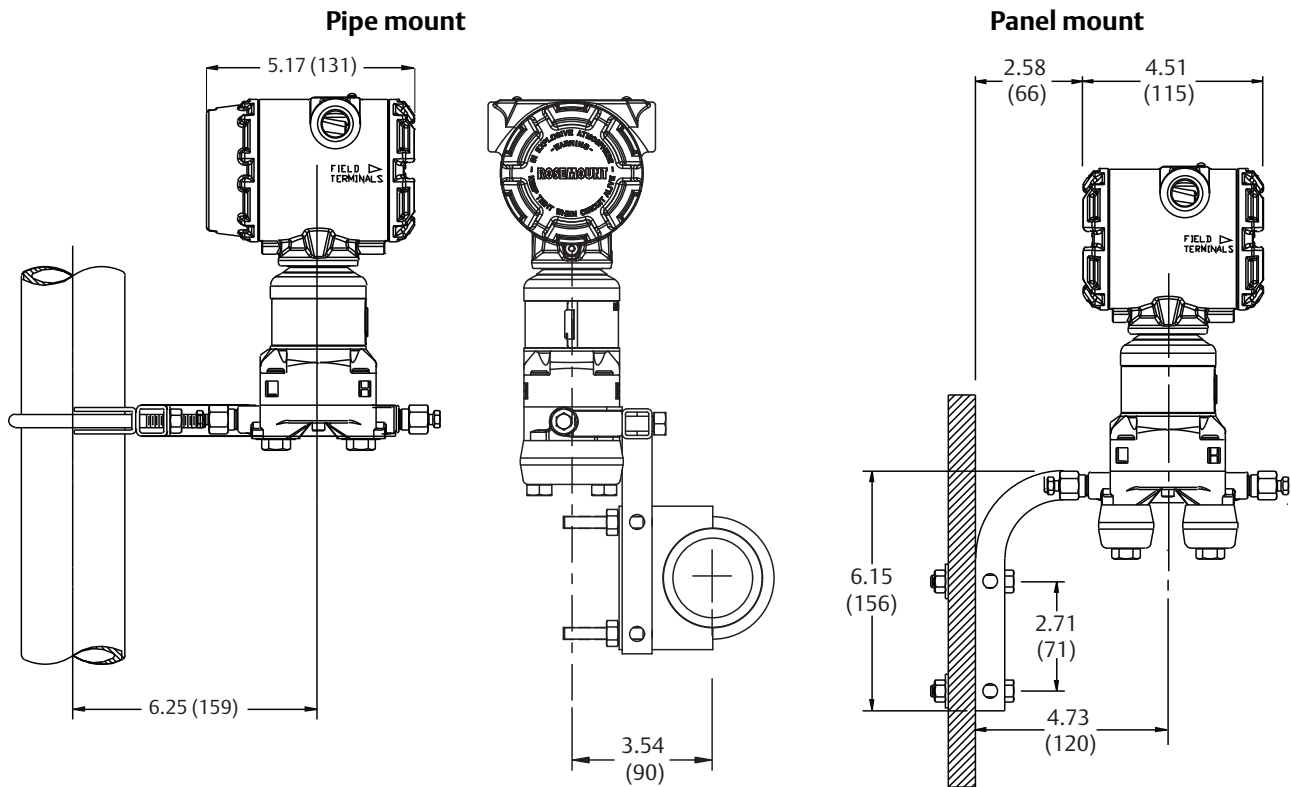
Figure 4. Coplanar Flange Mounting Configurations
