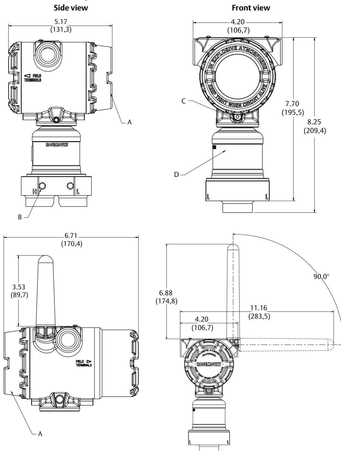
Figure 2. Plantweb Housing
