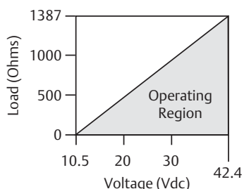
Figure 1. Rosemount 3051SHP
