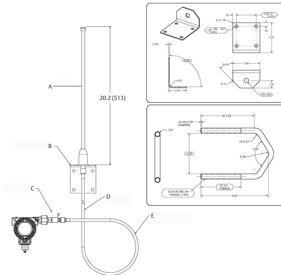
Figure 11: High Gain, Remote Mount Antenna (WN Option)
