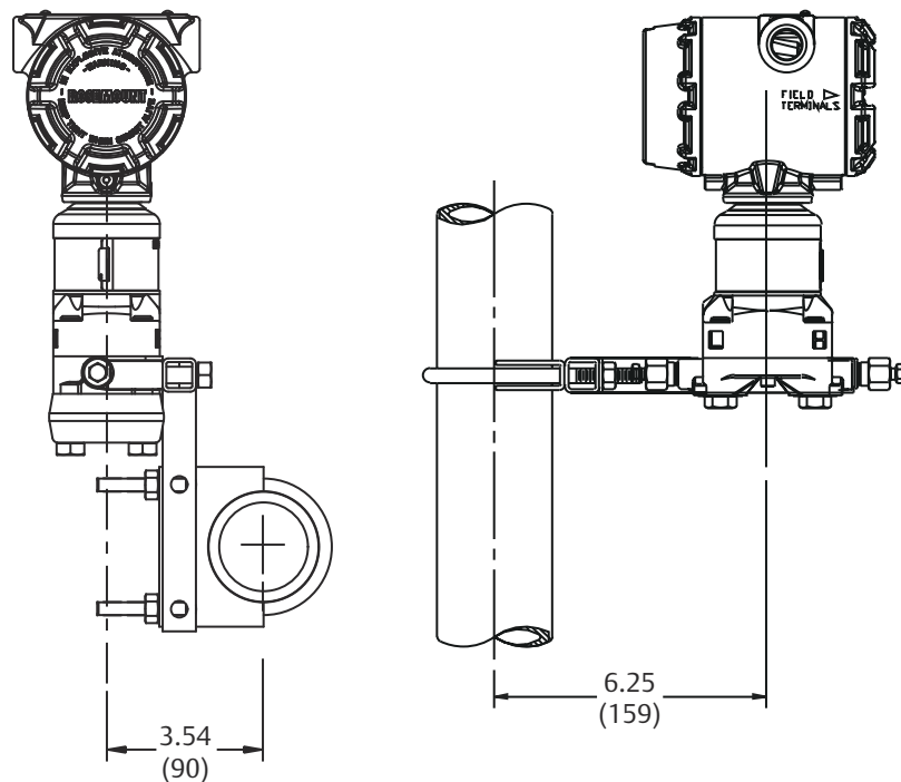
Figure 12: Coplanar Mounting Configurations (B4 Bracket)
