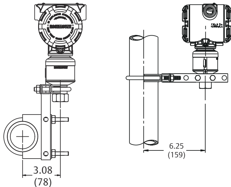
Figure 14: In-line Mounting Configurations (B4 Bracket)
