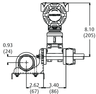
Figure 13: Traditional Mounting Configurations
