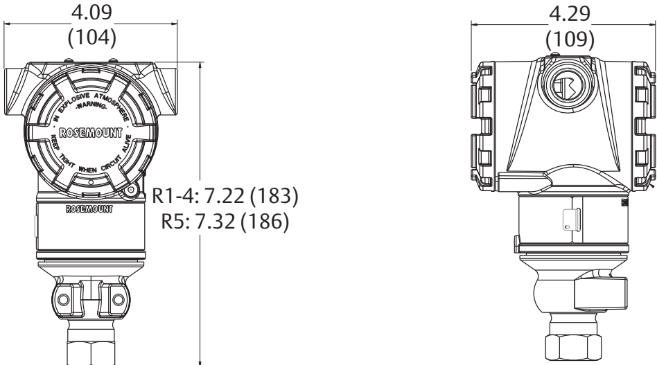
Figure 10. Rosemount 3051T Wireless Housing
