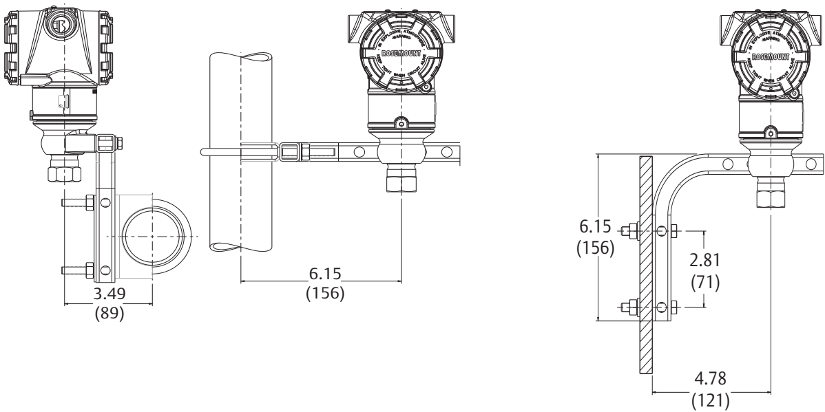
Figure 14. Rosemount 3051CFA Pak-Lok Annubar Flowmeter (1)
