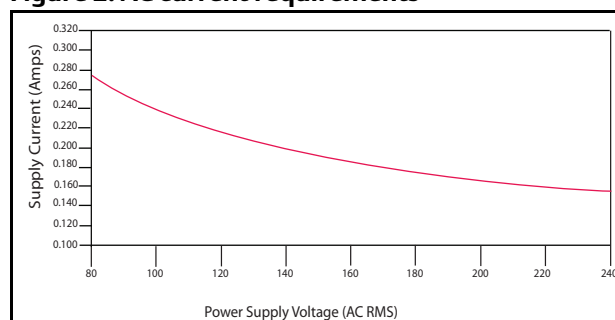
Figure 2. AC current requirements
