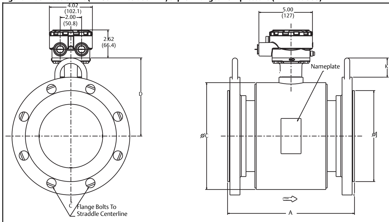
Figure 11. 3-in. to 36-in. (DN80 mm to 900 mm) slip-on flanges -low pressure ( P \leq \text{Class 300} )
