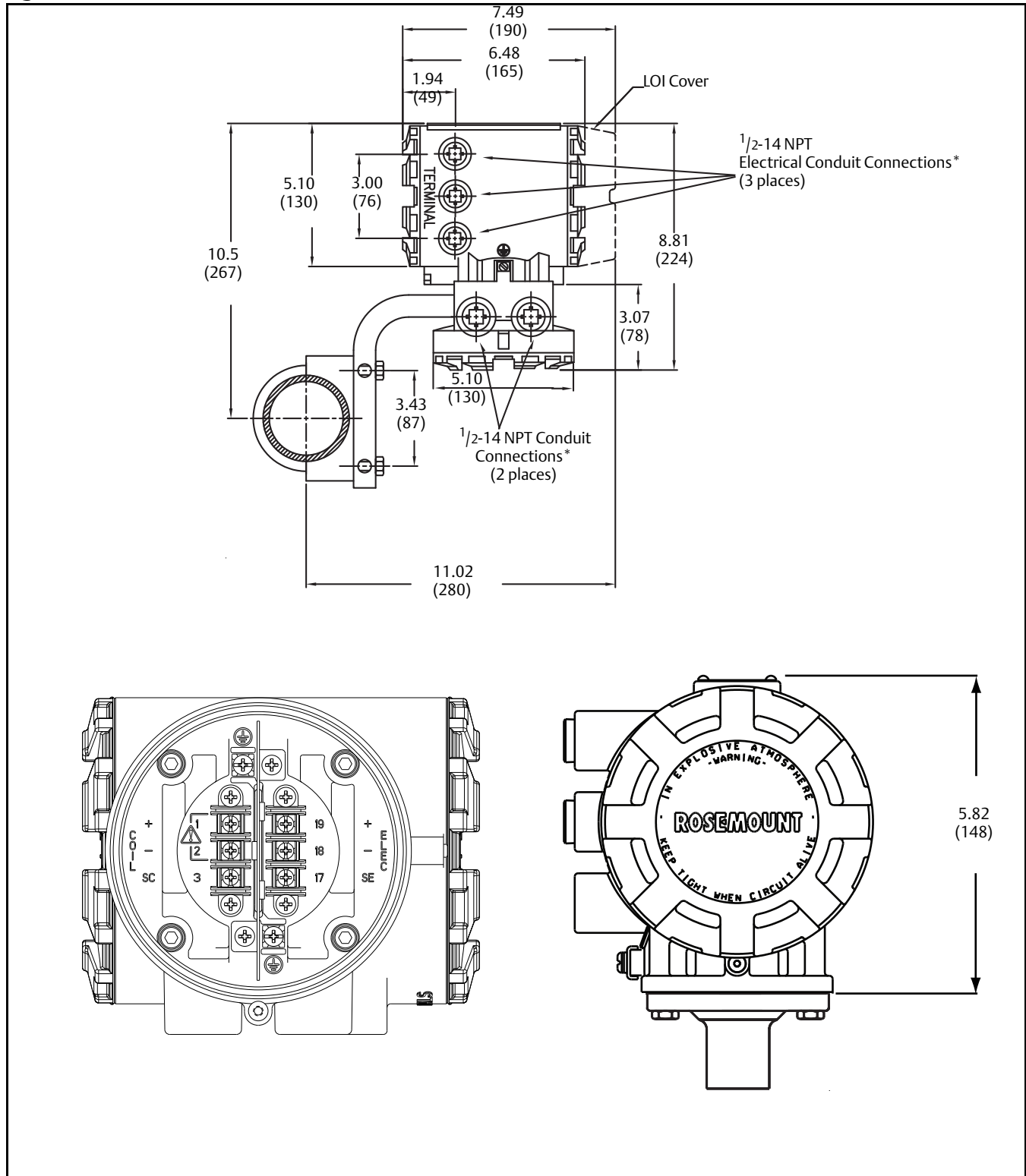
Figure 8. Rosemount 8732 Transmitter
