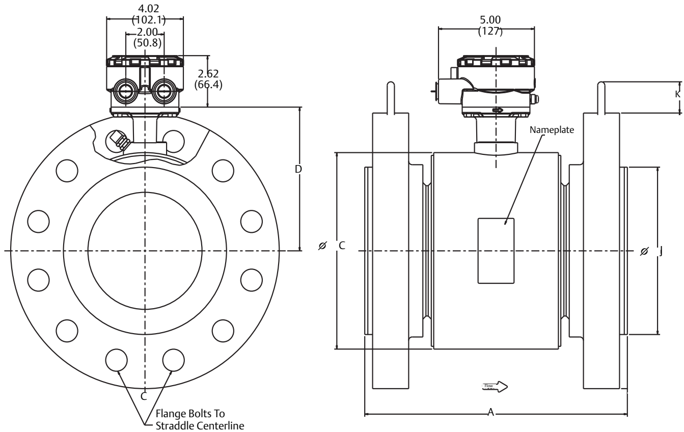
Figure 14. 1½-in. to 24-in. (DN15 mm to 600 mm) with slip-on flanges - high pressure meters (Class 600 - 900)
