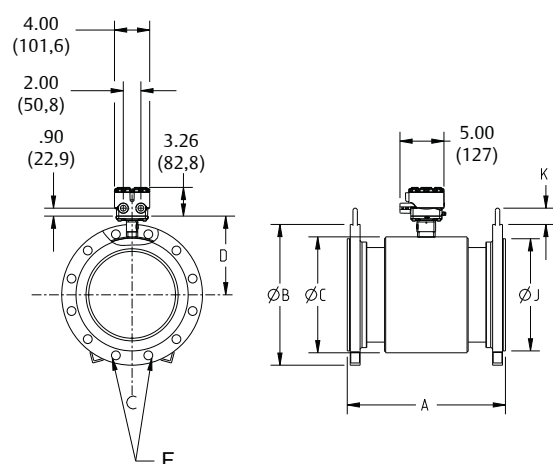
Figure 11: Raised face flanged sensor 3-in to 48-in. (75 mm to 1200 mm)
