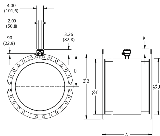
Figure 12: Flat face sensor 30- to 48-in. (750 mm to 1200 mm)
