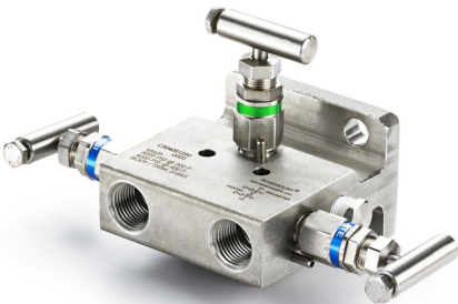
Rosemount 304 Conventional Manifold - Traditional Style
