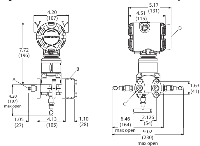
Figure 13. Rosemount 305RM 3-Valve Traditional DIN Style Manifold
