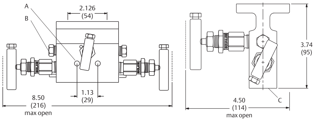
Figure 18. Rosemount 304RT 3-Valve Flange × NPT Conventional Manifold (1) Instrument side
