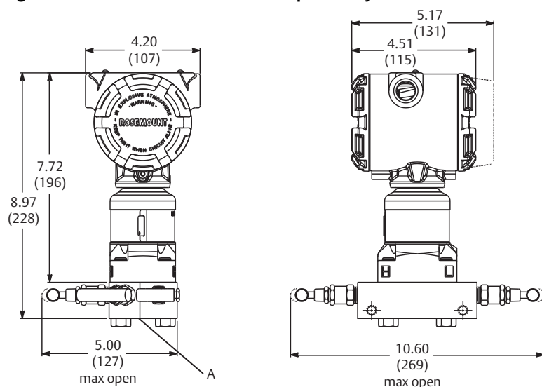
Figure 9. Rosemount 305RC 5-Valve Coplanar Style Manifold
