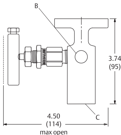
Figure 16. Rosemount 304RT 2-Valve Flange × NPT Conventional Manifold Instrument side
