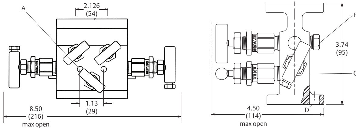
Figure 23. Rosemount 304RT Natural Gas 5-Valve Flange × Flange Conventional Manifold (1) Instrument side
