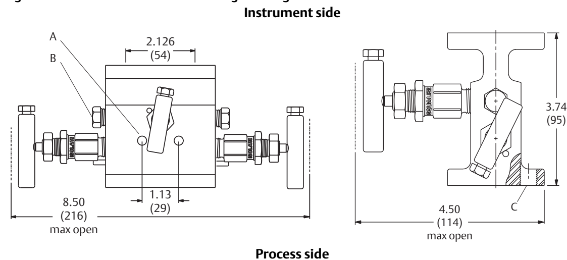
Figure 19. Rosemount 304RT 3-Valve Flange × Flange Conventional Manifold (1)
