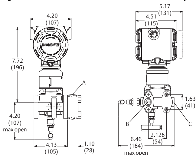
Figure 12. Rosemount 305RM 2-Valve Traditional DIN Style Manifold
