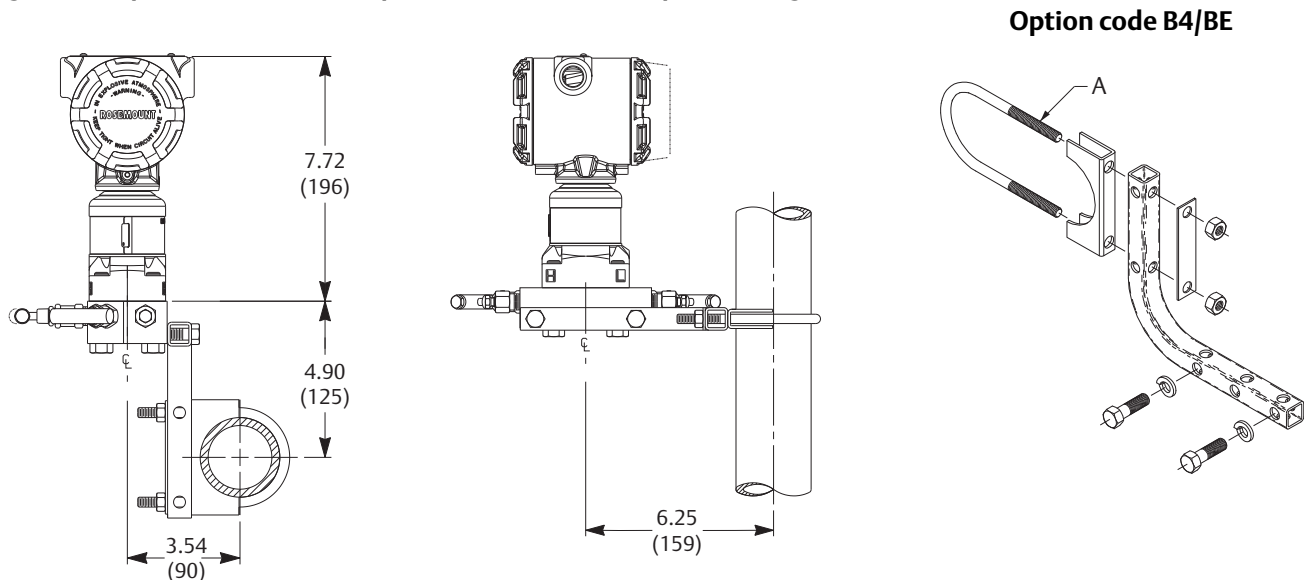
Figure 26. Coplanar Manifold with Optional Bracket for 2-in. Pipe Mounting (1)
