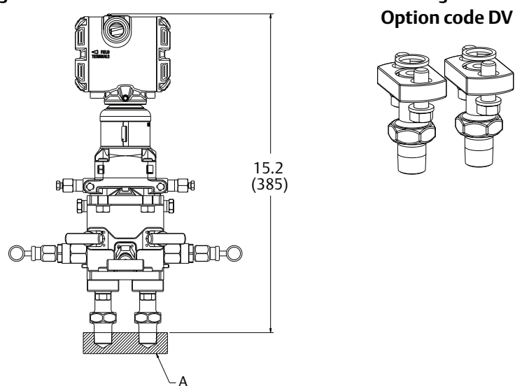
Figure 29. DV Non-Stabilized Connectors for Direct Mounting (1)(2)
