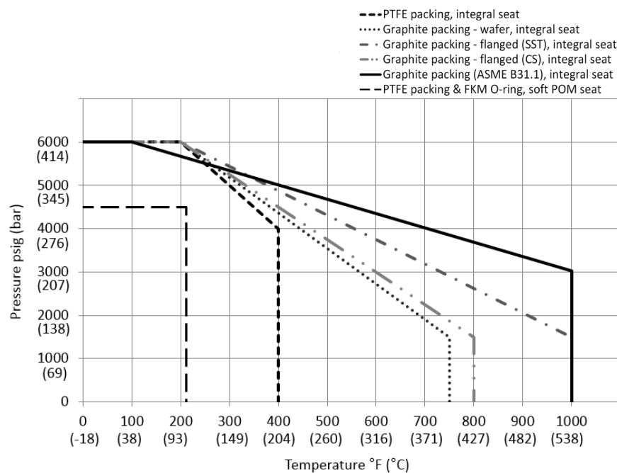
Figure 3. Rosemount 304 Conventional Manifolds
