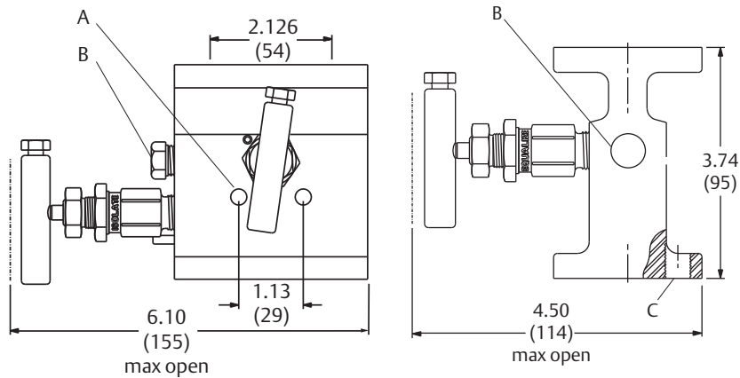
Figure 17. Rosemount 304RT 2-Valve Flange × Flange Conventional Manifold (1) Instrument side
