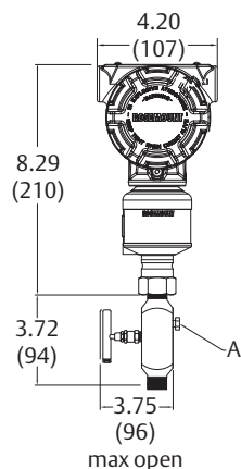
Figure 15. Rosemount 306RT Pressure Style Manifold (3051S_T Shown) (2)
