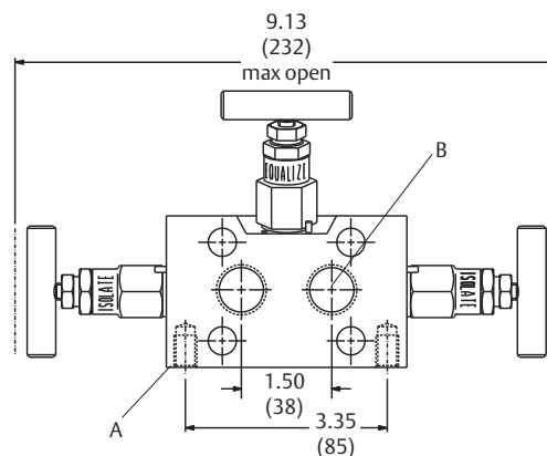
Figure 24. Rosemount 304RW 3-Valve Wafer Manifold (1)
