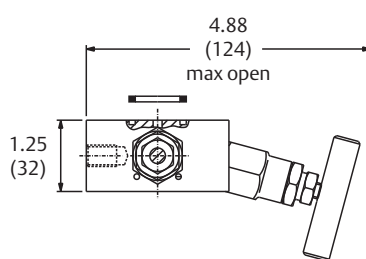
Figure 24. Rosemount 304RW 3-Valve Wafer Manifold (1)
