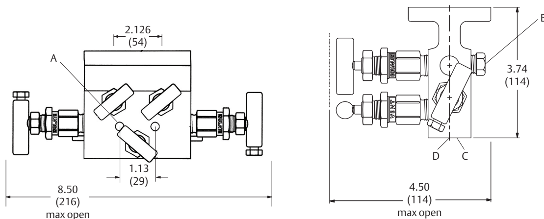
Figure 22. Rosemount 304RT Natural Gas 5-Valve Flange × NPT Conventional Manifold (1) Instrument side
