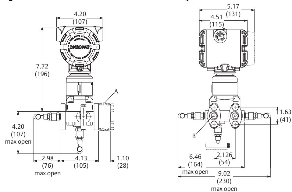
Figure 14. Rosemount 305RM 5-Valve Traditional DIN Style Manifold
