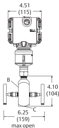
Figure 15. Rosemount 306RT Pressure Style Manifold (3051S_T Shown) (2)
