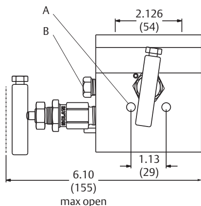
Figure 16. Rosemount 304RT 2-Valve Flange × NPT Conventional Manifold Instrument side
