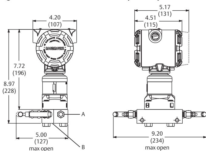
Figure 8. Rosemount 305RC 3-Valve Coplanar Style Manifolds
