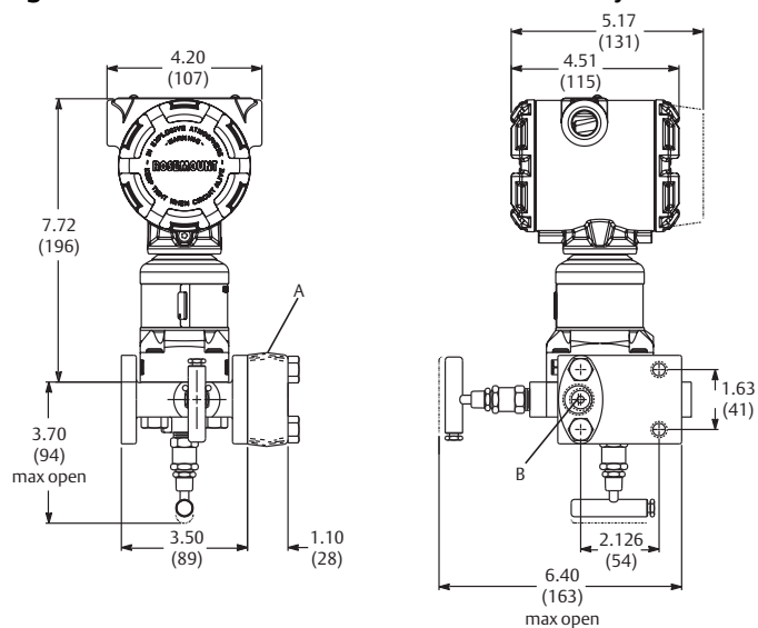
Figure 10. Rosemount 305RT 2-Valve Traditional Style Manifold
