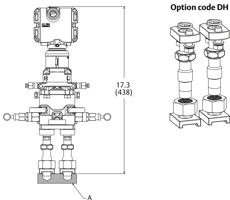
Figure 28. DH Extended Stabilized Connectors for Direct Mounting (1)(2)
