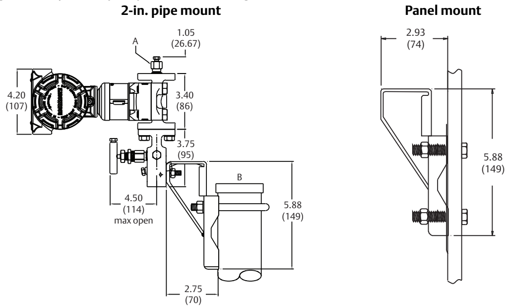
Figure 27. VS/VC Heavy Duty Manifold Mounting Bracket (1)
