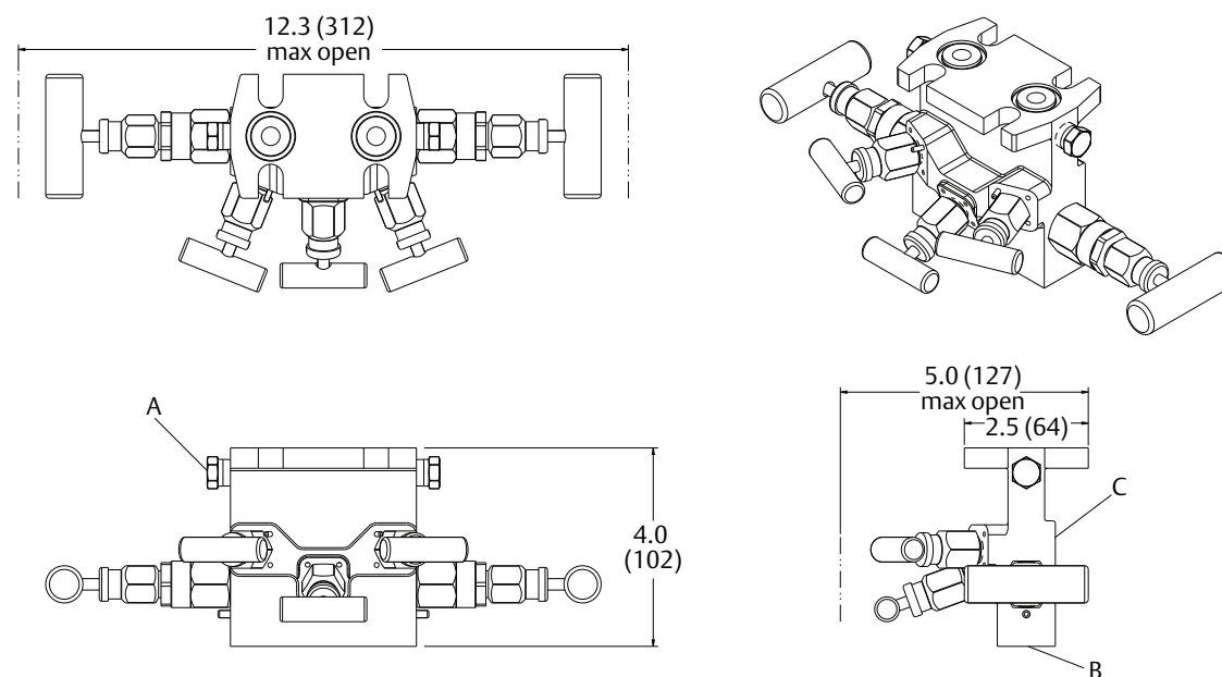
Figure 20. Rosemount 304RT Natural Gas 5-Valve Flange × NPT Conventional Manifold with NG Option
