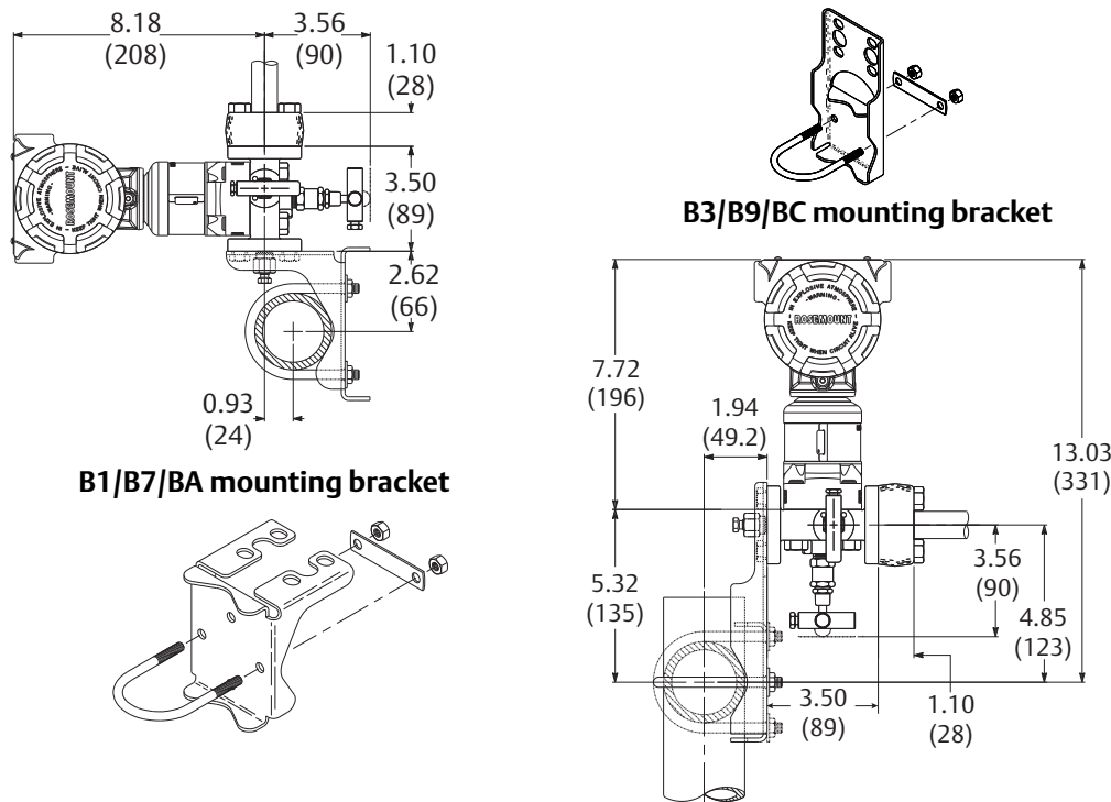
Figure 25. Traditional Manifold with Optional Brackets for 2-in. Pipe Mounting (1)
