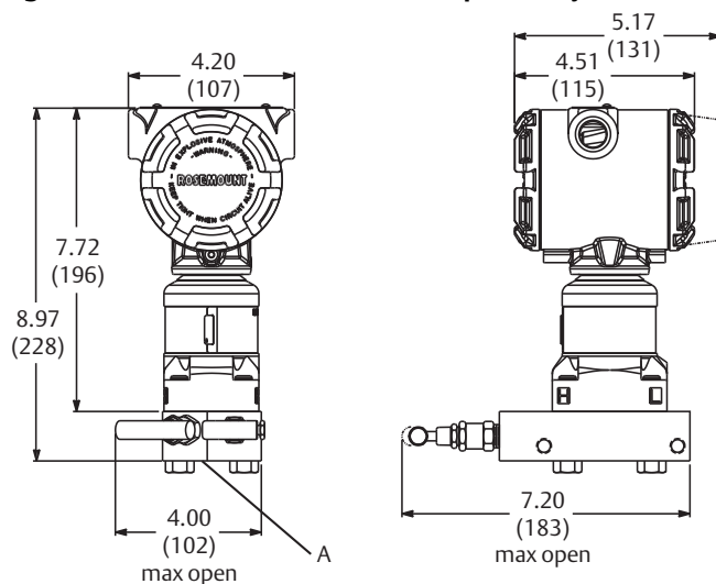
Figure 7. Rosemount 305RC 2-Valve Coplanar Style Manifold
