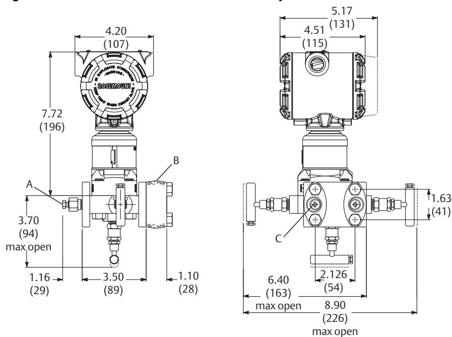
Figure 11. Rosemount 305RT 3-Valve Traditional Style Manifold
