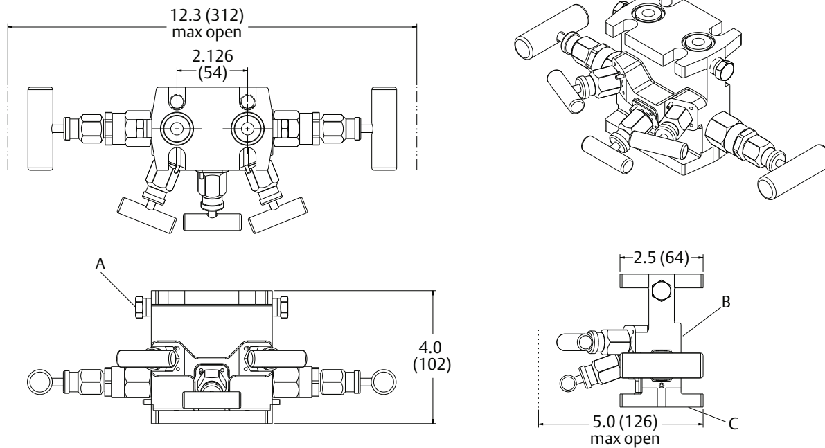
Figure 21. Rosemount 304RT Natural Gas 5-Valve Conventional Manifold with NG Option
