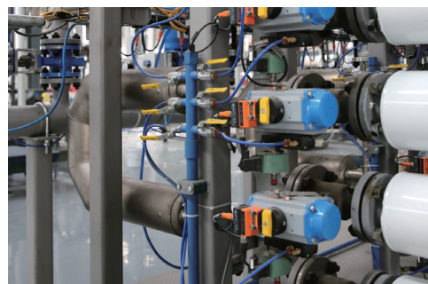
Emerson's Simultaneous Metered Blenders are equipped with our Micro Motion ELITE® Coriolis flow meters to ensure high accuracy blending. Photo courtesy of Copton.
