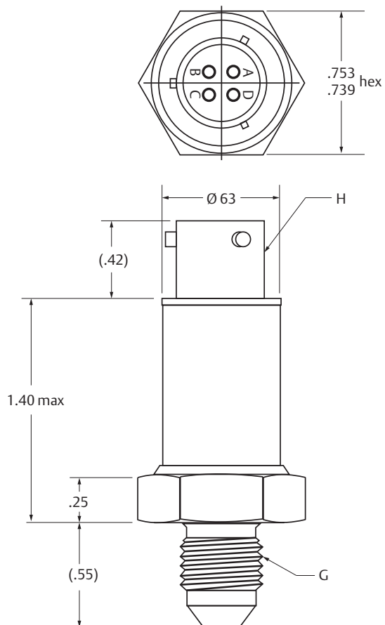
Figure 1. Paine 210-30-110 Series
