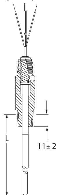
Figure 3. 1/2-in. ANPT Spring Loaded Adapter
