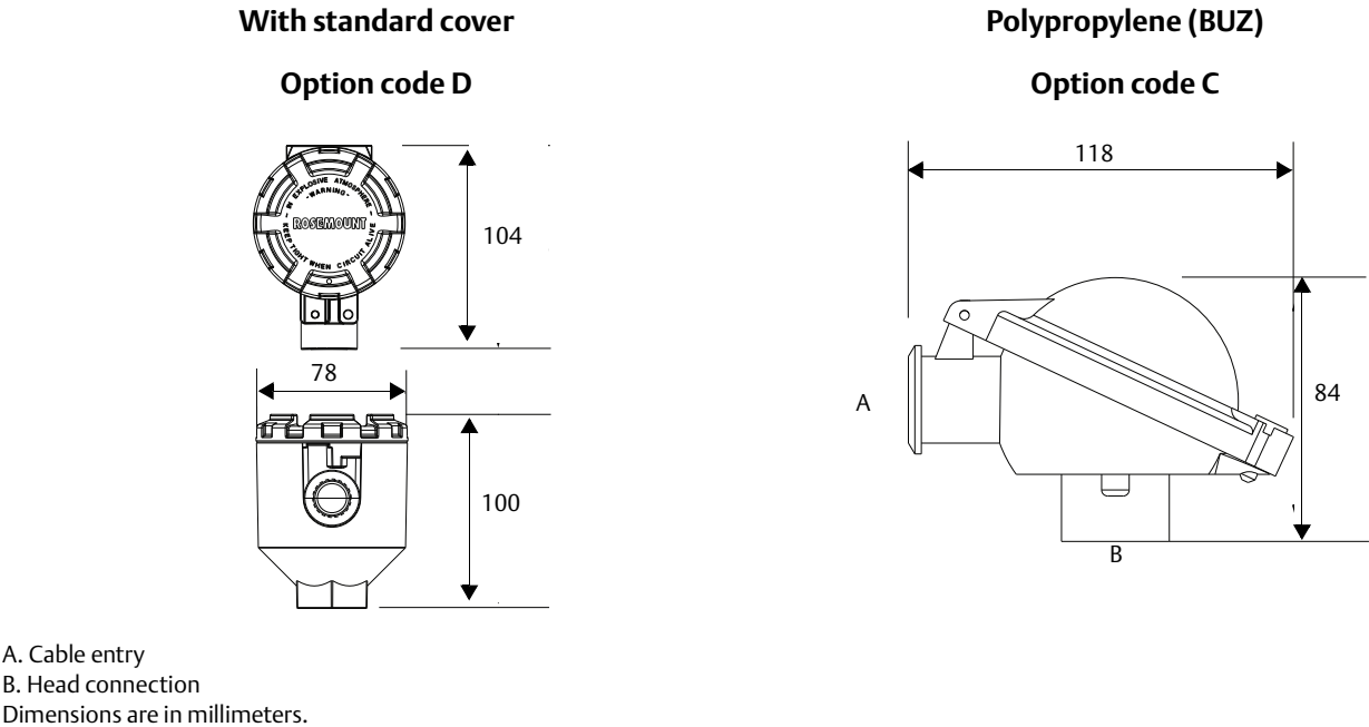
Figure 9. Connection Head Dimensional Drawing
