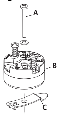
A. Mounting Hardware B. Transmitter C. Rail Clip
