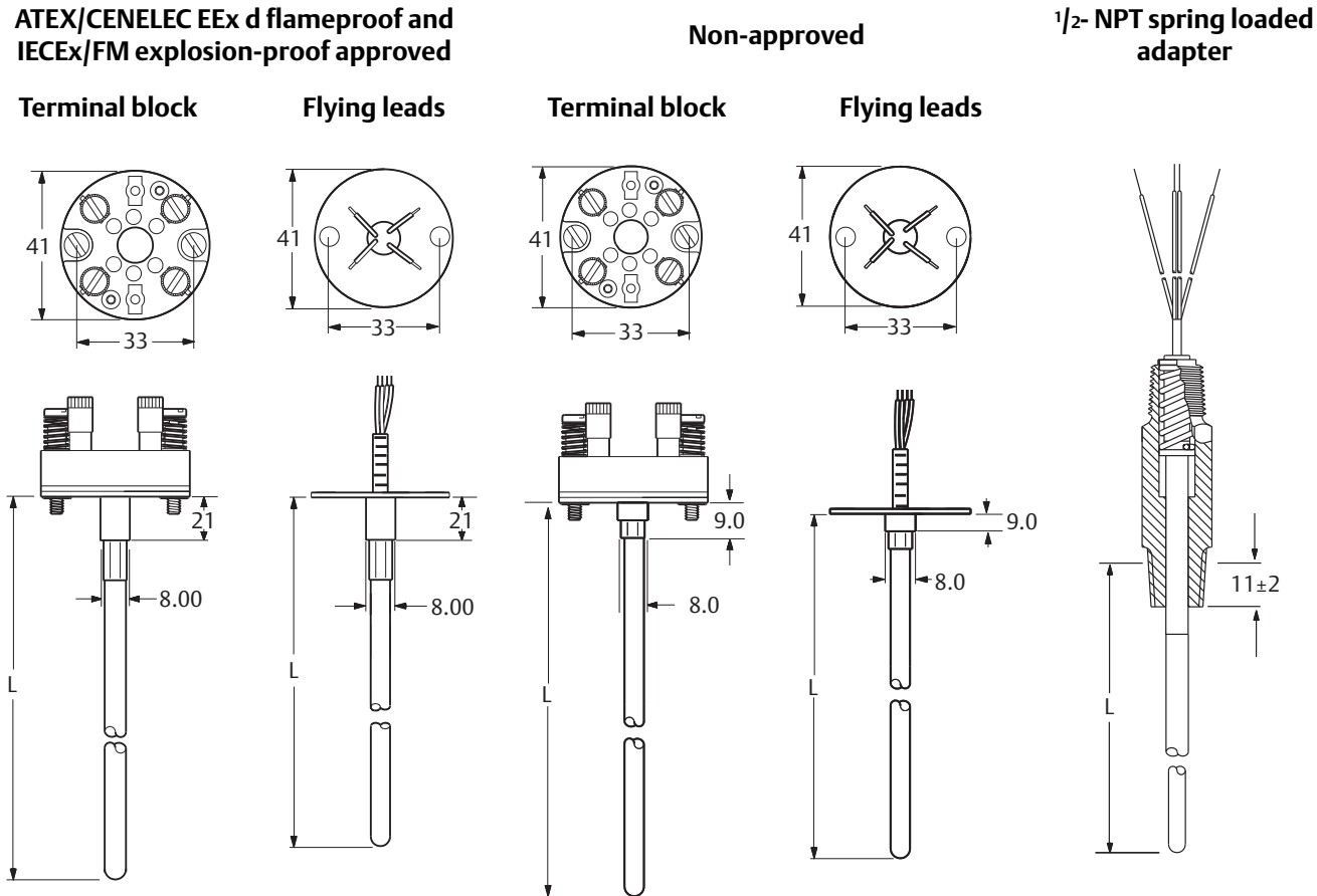
Figure 6. Series 65 RTD and Series 185 Thermocouple Dimensional Drawings
