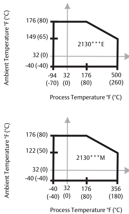
Figure 2. Operating Temperatures
