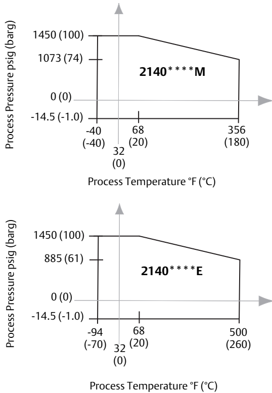
Figure 1. Operating Pressures
