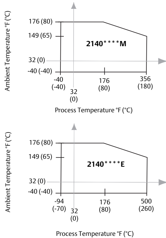
Figure 2. Operating Temperatures
