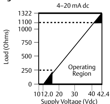
Figure 1. Maximum Load = 40.8 \times (\text{Supply Voltage} - 12.0)
