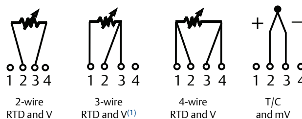
Figure 2. Rosemount 248 Sensor Connections
