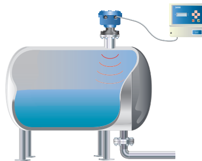
Level measurement with a Rosemount 3100 Series transmitter and Rosemount 3490 Controller Unit
