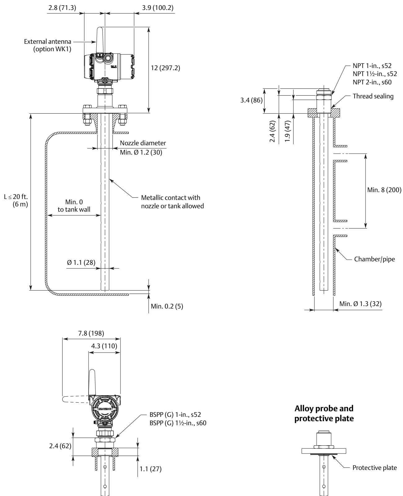
Figure 18. Coaxial Probe
