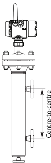
Side-and-side dimension
