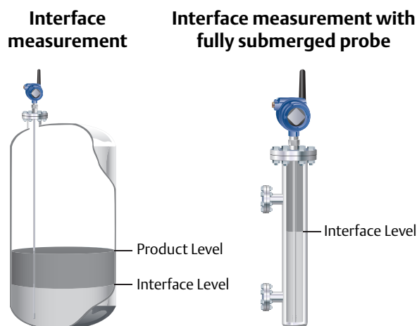
Figure 8. Interface Measurements
