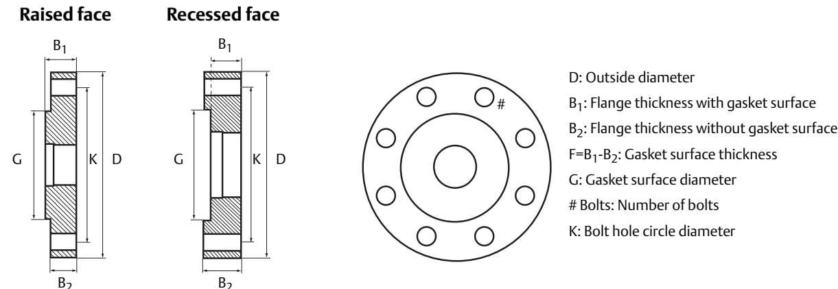
Figure 22. Proprietary Flanges
