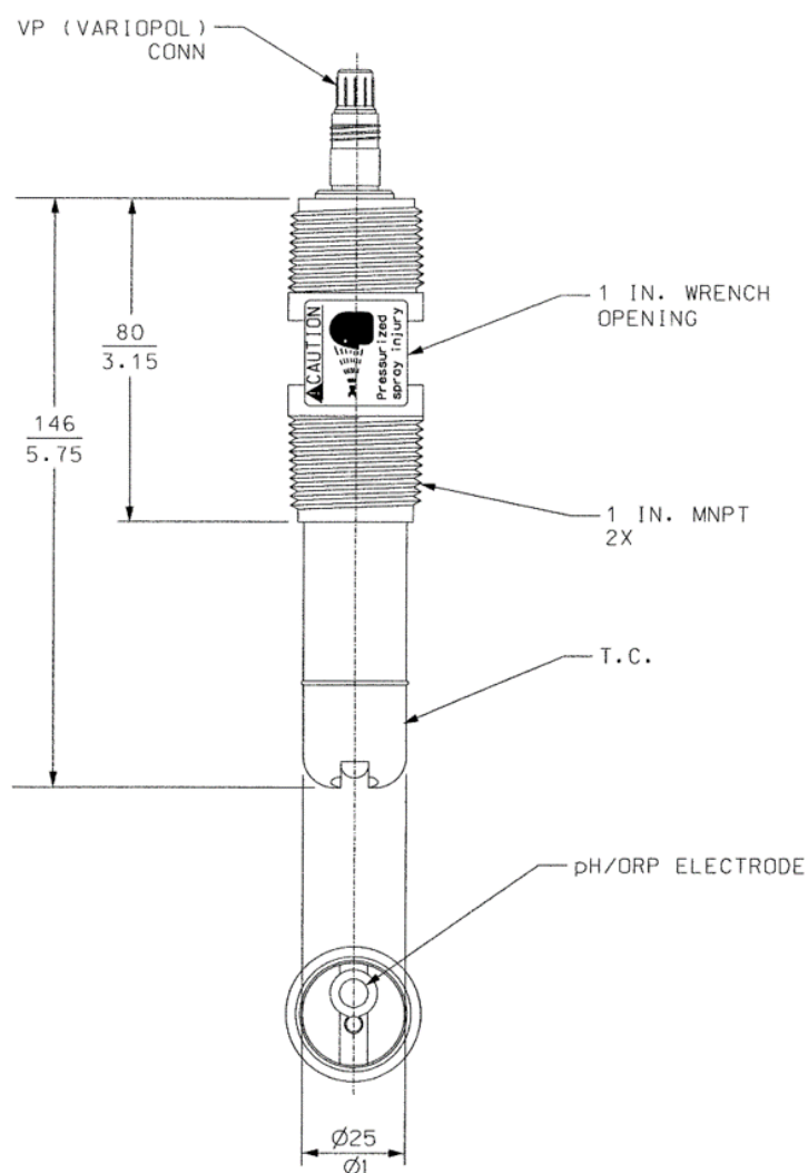
Figure 3. Rosemount 389VP with Variopool cable connection dimensional drawing
