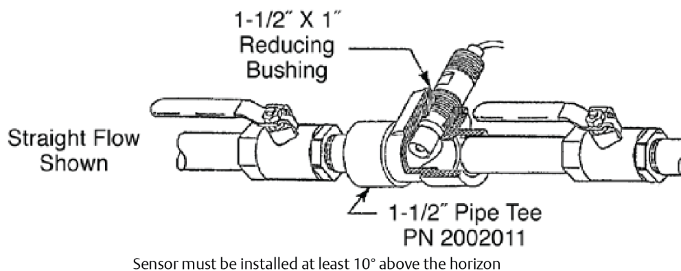
Figure 3. Typical flow through insertion installation using PN 2002011 pipe tee
