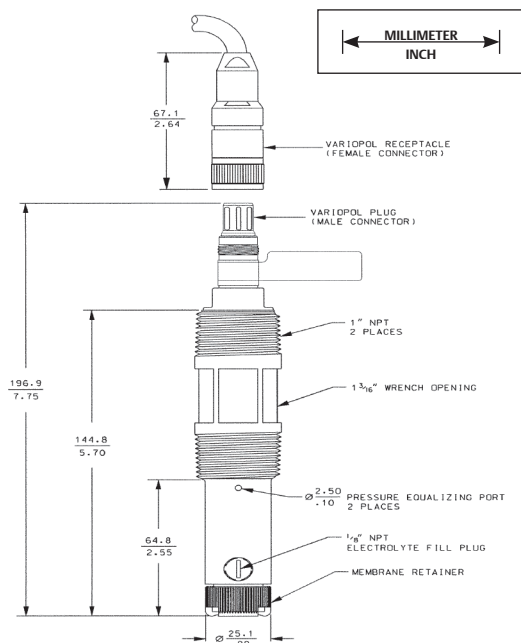
Figure 2 Sensor with Variopol connector.
