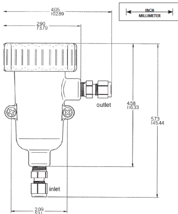
Figure 3 Low flow cell (PN 24091-00)
