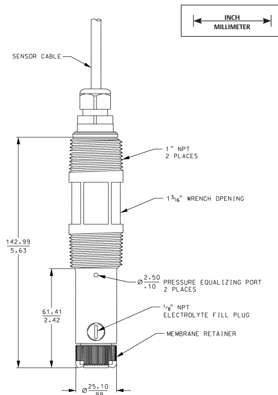
Figure 1. Rosemount 499AOZ with Integral Cable Sensor dimensions
