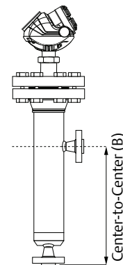
Side-and-Bottom dimension
