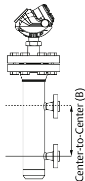
Side-and-Side dimension
