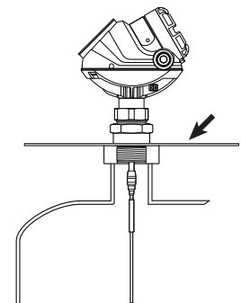
Metal sheet ( d > 14 in./350 mm)
