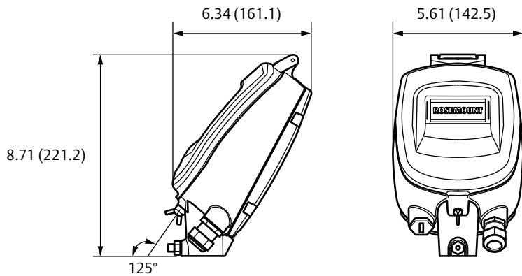
Figure 3. Rosemount 5708 Housing
