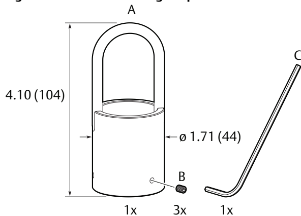
Figure 9. Manhole Mounting Adapter
