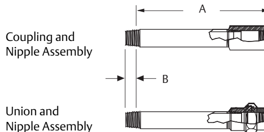
Figure 27. Extension Fitting
