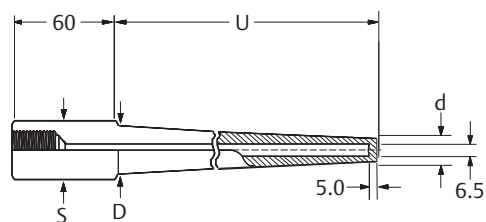
Figure 13. Weld-In Barstock Thermowell (Codes W10, W12, W14, W16)
