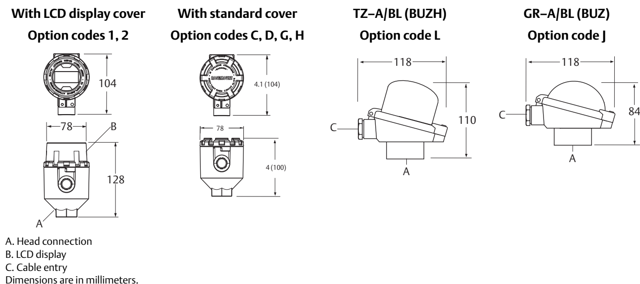
Figure 9. Connection Head Dimensional Drawing
