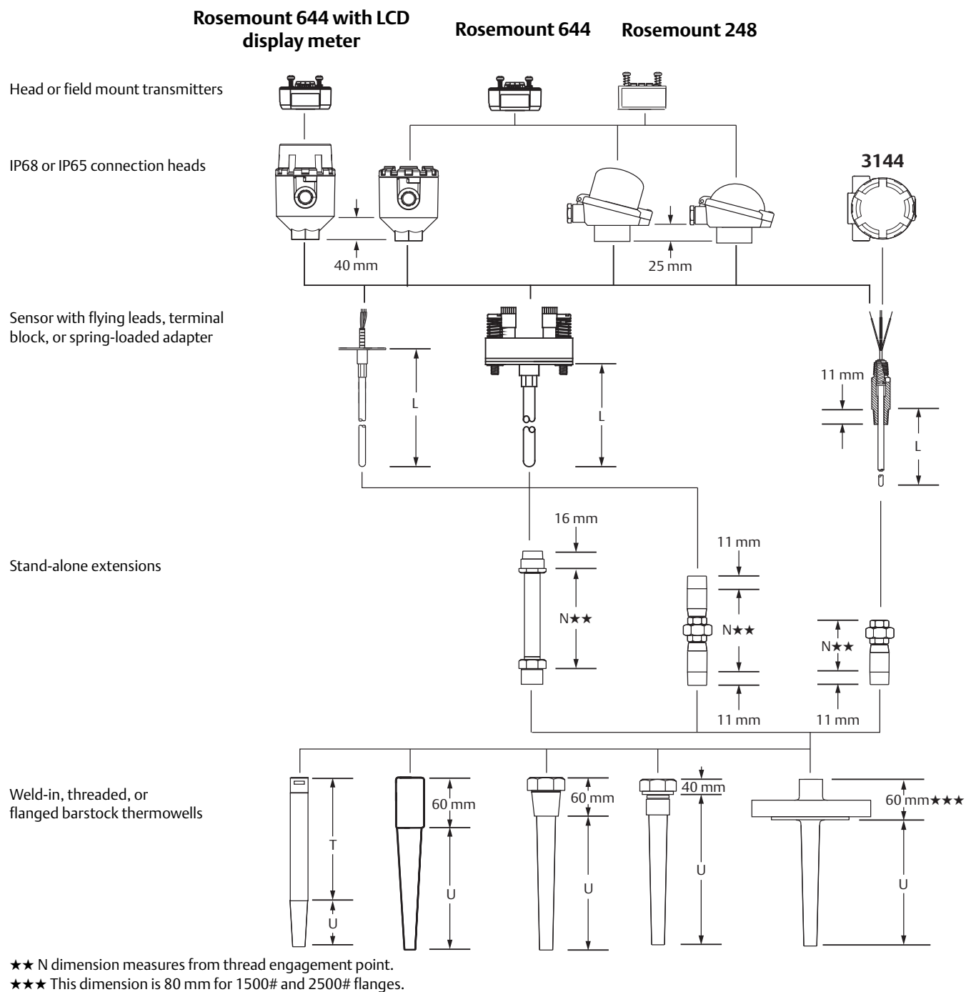
Figure 8. Barstock Thermowell Sensor Assemblies
