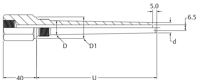
Figure 11. Threaded Barstock Thermowell – Parallel Thread
