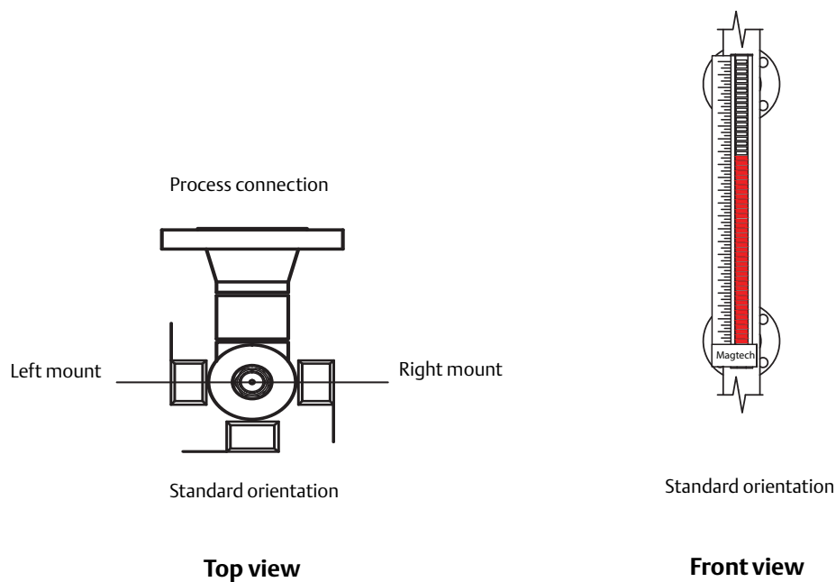
Figure 2. Indicator/Scale Orientation
