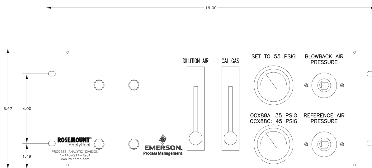
Auto-calibration panel
