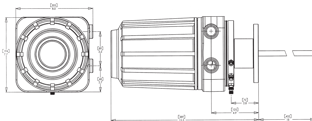
Sensor Housing
