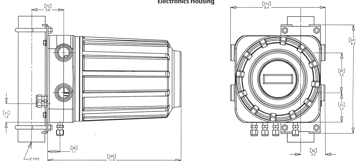
Electronics Housing
