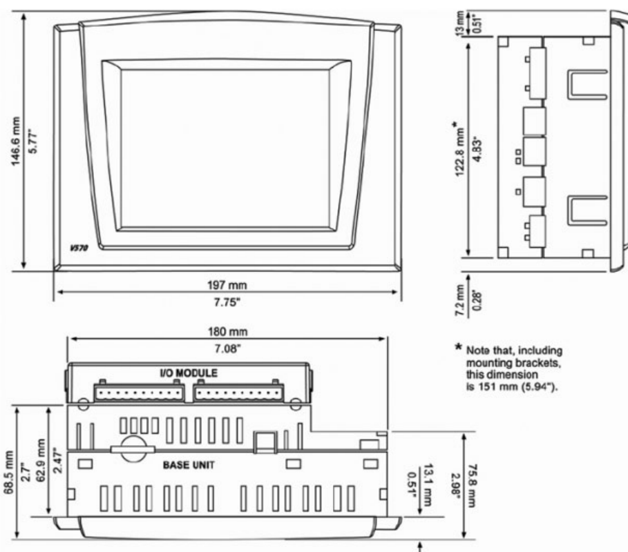
OPM 4001 Enhanced Control Unit
