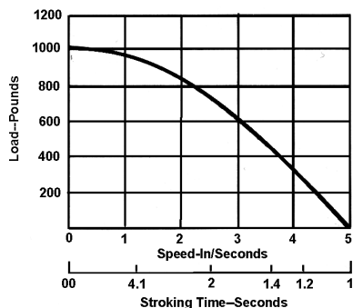
Speed-Thrust Curve
